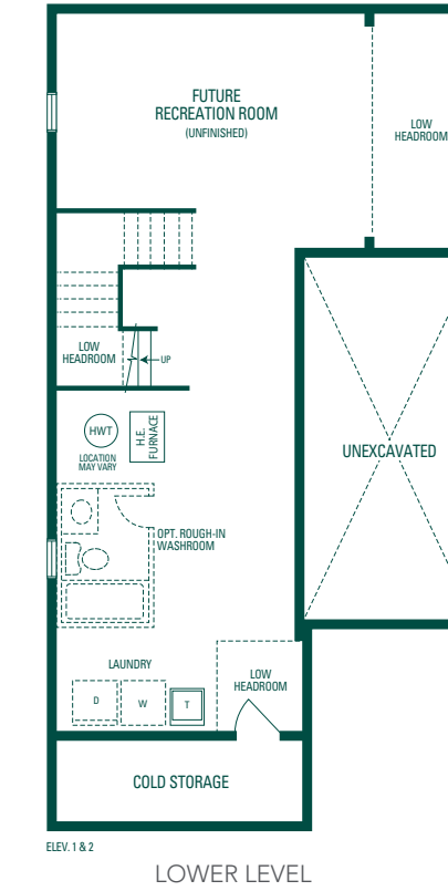
LOWER LEVEL
