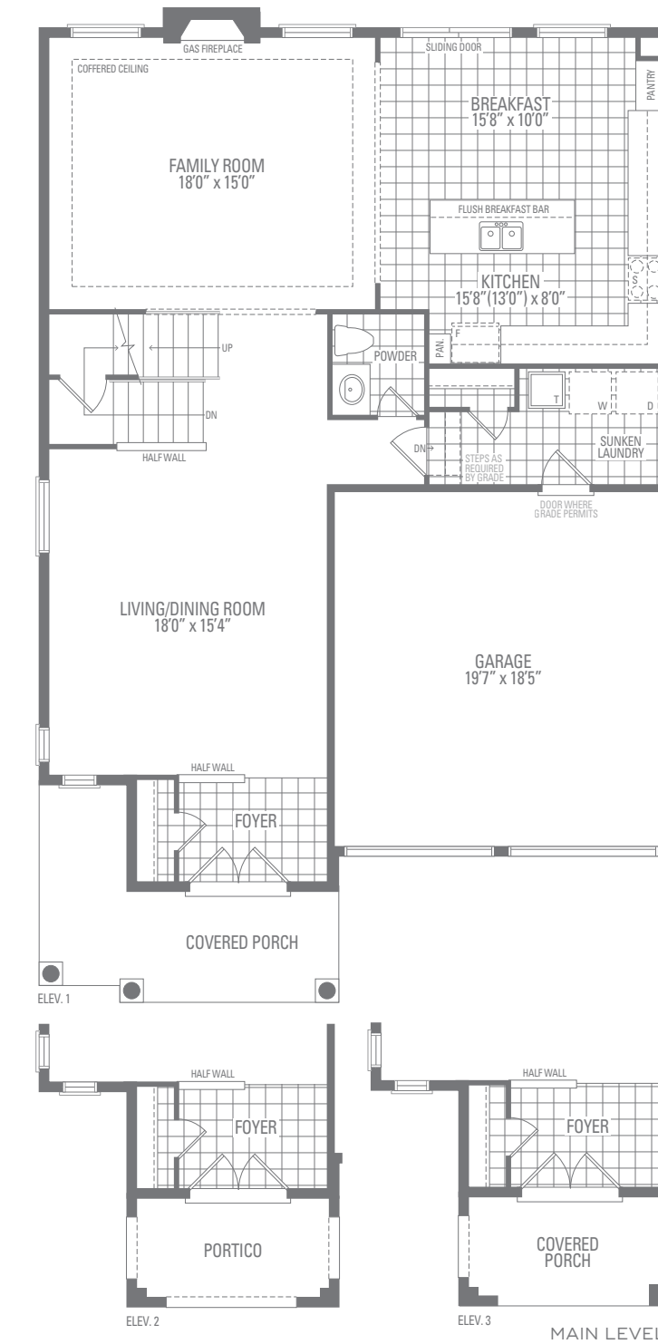
MAIN LEVEL
