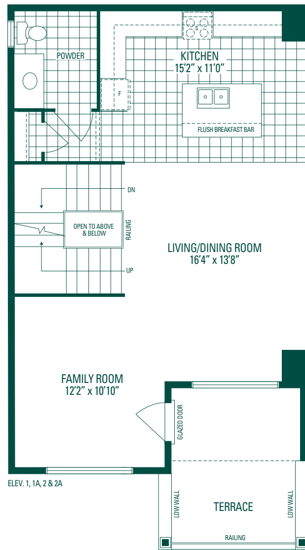
MAIN LEVEL
